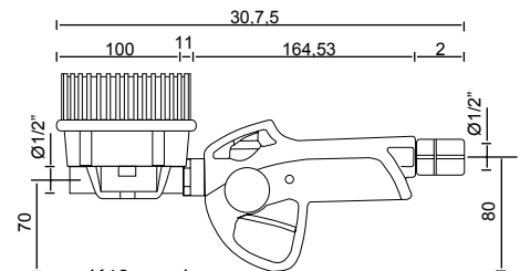
K40 nozzle
